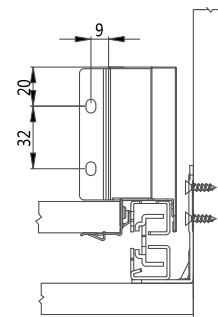
Rear Plate Mounting Dimensions
