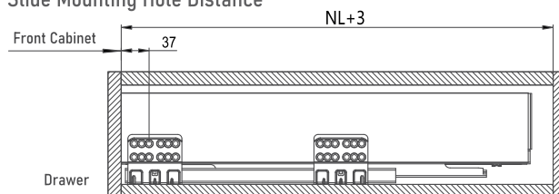
Slide Mounting Hole Distance
