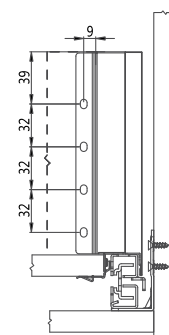
Rear Plate Mounting Dimensions
