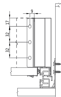
Rear Plate Mounting Dimensions
