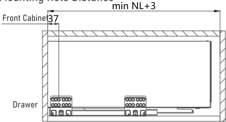
Slide Mounting Hole Distance
