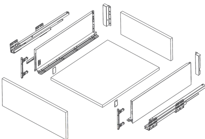
Assembly
