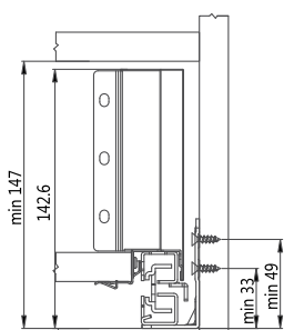
Cabinet Space Dimension
