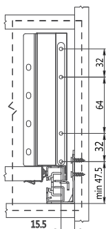
Front Panel Connector Mounting Dimensions
