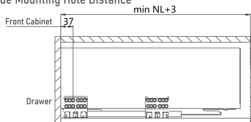
Slide Mounting Hole Distance
