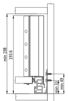
Cabinet Space Dimension
