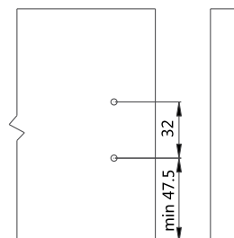
Panel Dimensions
